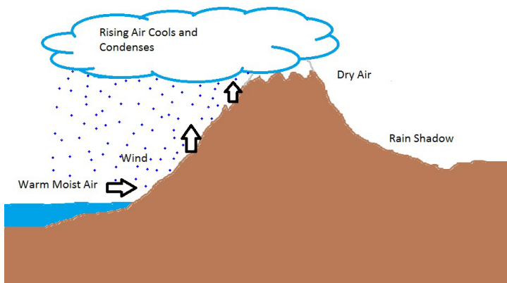
Figure 2. Adiabatic cooling: moist ocean air is lifted uphill over elevated ground, cooling and shedding moisture as it rises. Over the mountain, then, air moving downhill warms and dries as it returns to lower elevation, producing a rain shadow .
