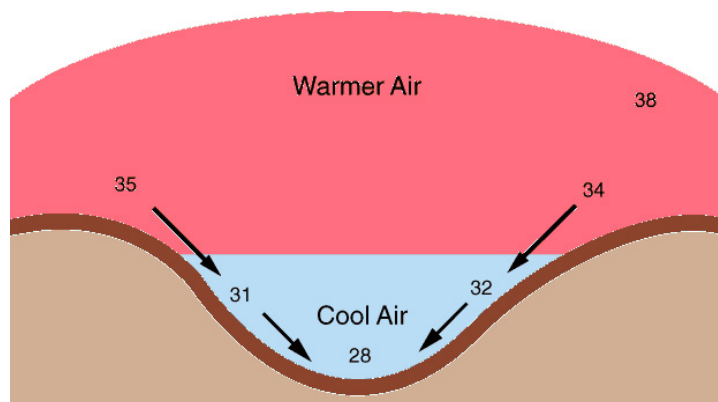
Figure 1. Static cold air in a cold sink can produce atypical-for-zone frost (Mass 2008). The numbers in this diagram refer to temperatures (F) as they “sink” into a sub-freezing area.
